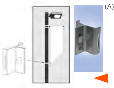
Tie-Down Bracket
