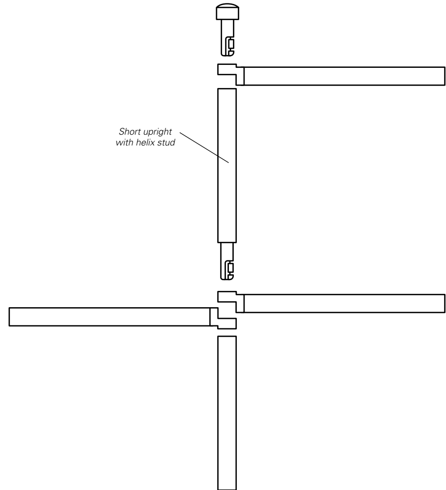
Blowup of section of DisplayONE unit; not to scale
